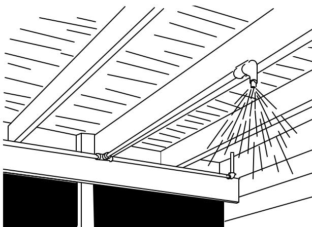
Figure 8. Sprinkler installed in a livestock building. From Fire Control In Livestock Buildings , NRAES-39.
