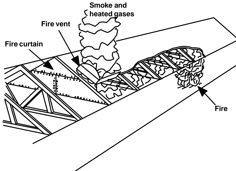
Figure 4. A fire curtain to delay and limit the horizontal spread of heat, smoke, and flame. From Fire Control In Livestock Buildings , NRAES-39.
