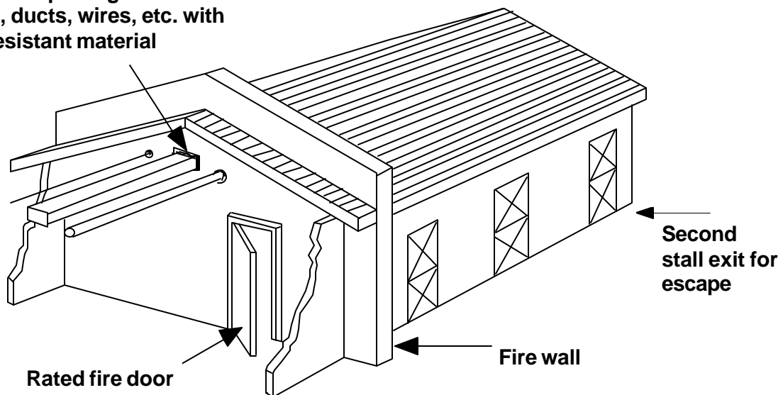
Figure 3. Fire wall to prevent or delay the spread of fire. From Fire Control In Livestock Buildings , NRAES-39.
